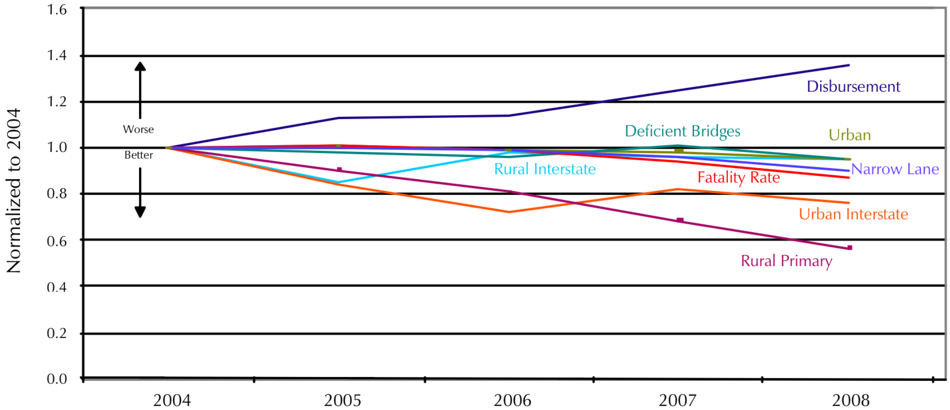
Figure 1: Trends in U.S. Highway Performance
