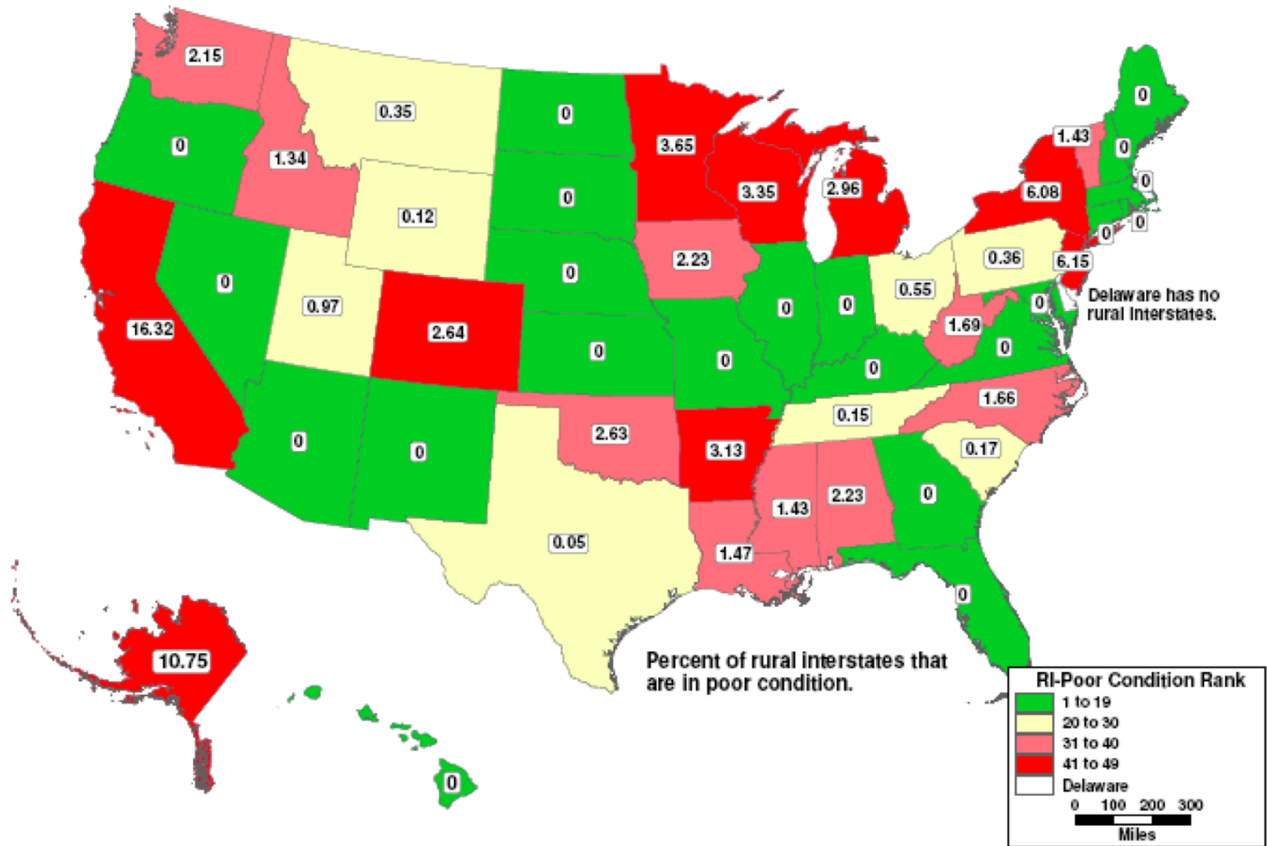
Figure 4: Percent of Rural Interstates in Poor Condition, 2008
